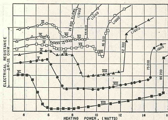
Fig. 9. Resistance changes associated with various phase changes in Bi.
