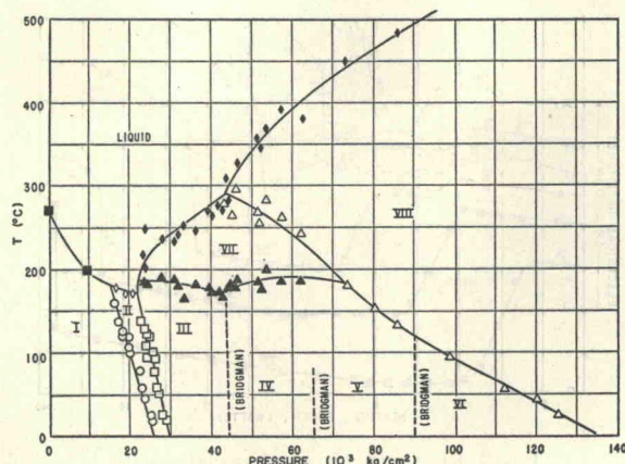
FIG. 5. Phase diagram for Bi.
