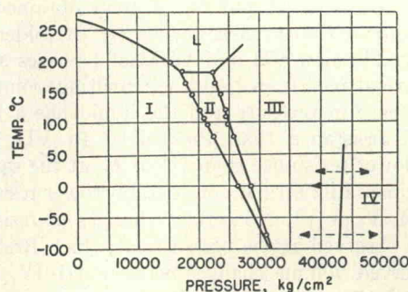
FIG. 1. Phase diagram of Bi (Bridgman).
