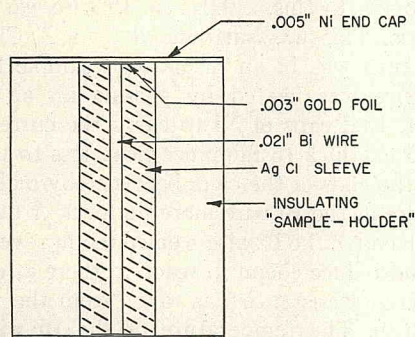
FIG. 2. Simple directly heated cell.
