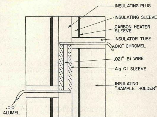
FIG. 3. Bi phase cell with indirect heating and chromel-Bi-alumel thermocouple.
