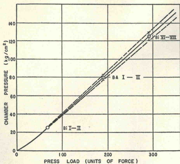
FIG. 11. Chamber pressure vs press load for superpressure apparatus.
