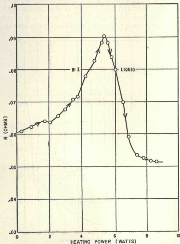
FIG. 6. Resistance change upon melting Bi I at 7800 kg/cm 2 .
