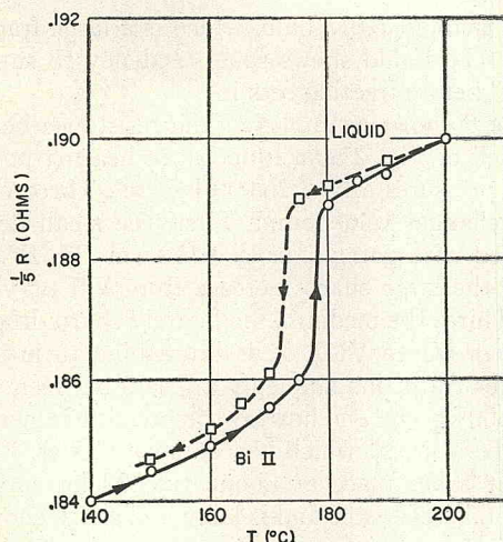
Fig. 8. Resistance change associated with Bi II \rightarrow liquid.
