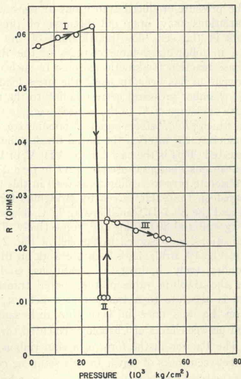
FIG. 7. Resistance changes associated with Bi I-II and Bi II-III at 25°C.
