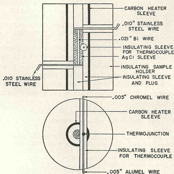
FIG. 4. Bi phase cell with indirect heating and independent thermocouple.
