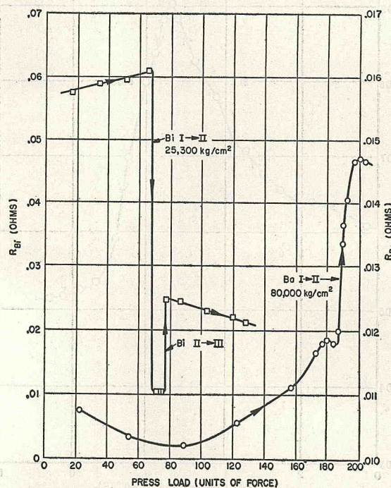
Fig. 10. Pressure calibration of cell by Bi and Ba transitions.
